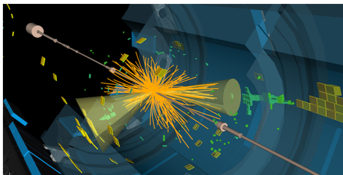
Figure 1: Display of a proton–proton collision event recorded at the ATLAS detector in 2022. ATLAS has now characterized the decay of Higgs bosons into muon–antimuon pairs, confirming previous measurements by the CMS Collaboration.
